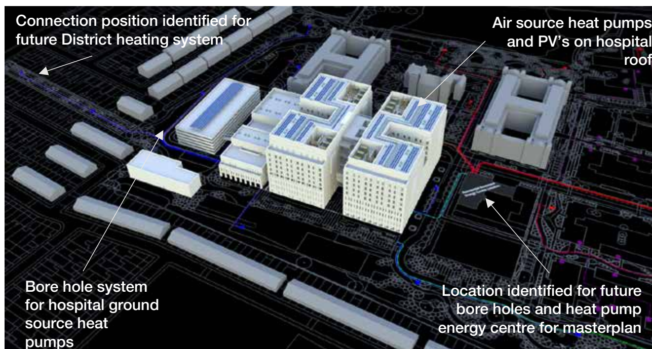
Whipps Cross Hospital renewable energy and heat networks
