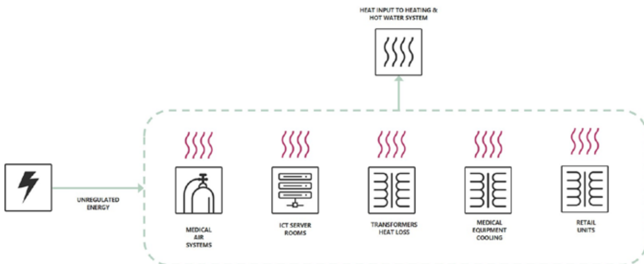
The Heat Wrap principle
