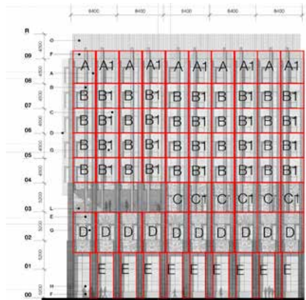
Early study for standard external envelope panel types on a typical elevation
