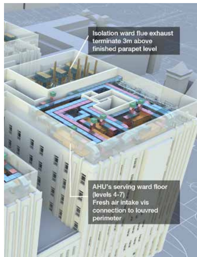
Ward ventilation strategy
